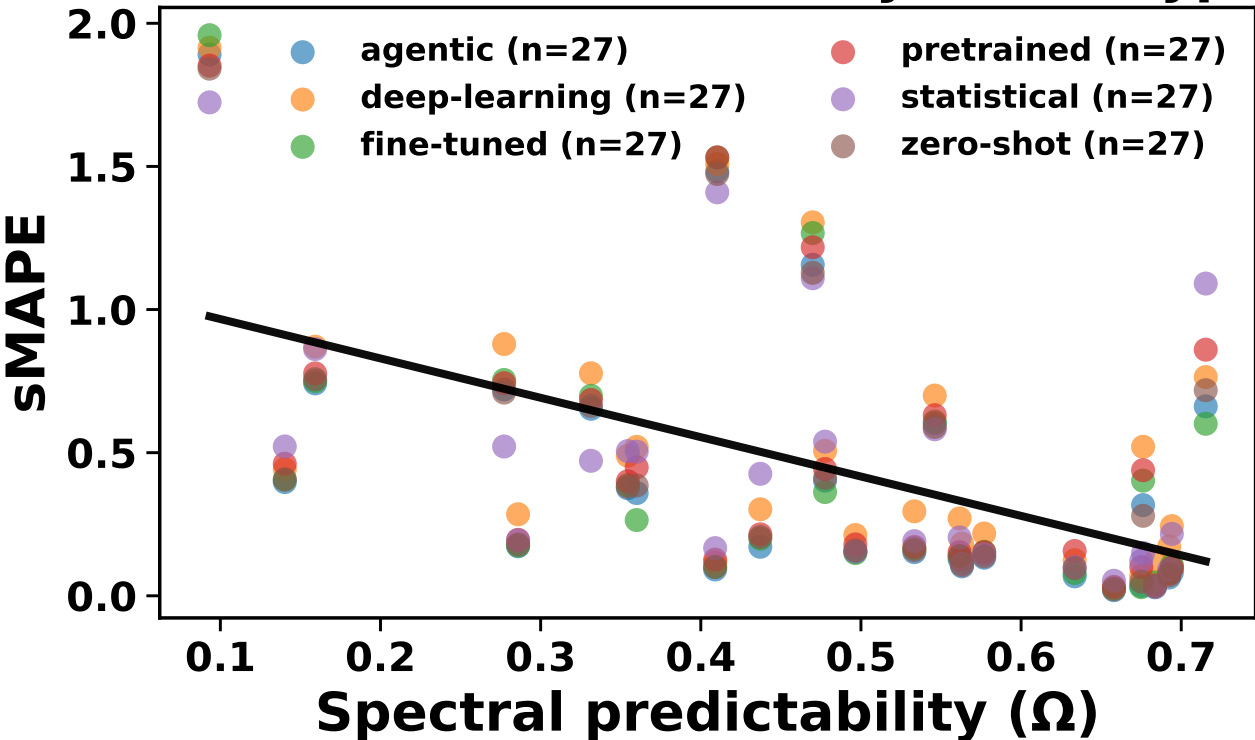
\Omega vs sMAPE — Colored by Model Type
